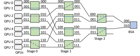
Fig. 3: 8-input QTS.
